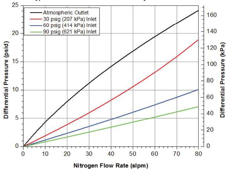
Mott POU-3-S Flow Rate vs. Differential Pressure Typical Flow Curves as a Function of System Pressures
