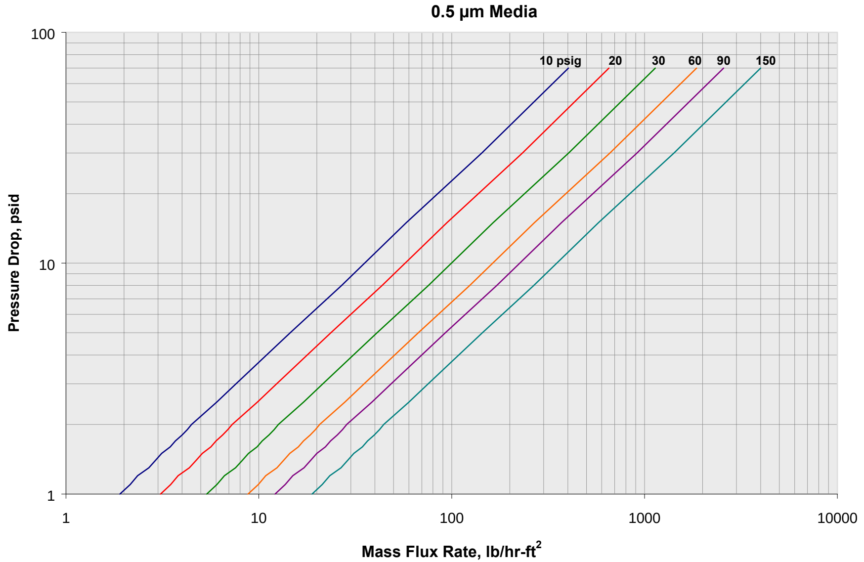
Figure 5: Media Pressure Drop by Steam Pressure
