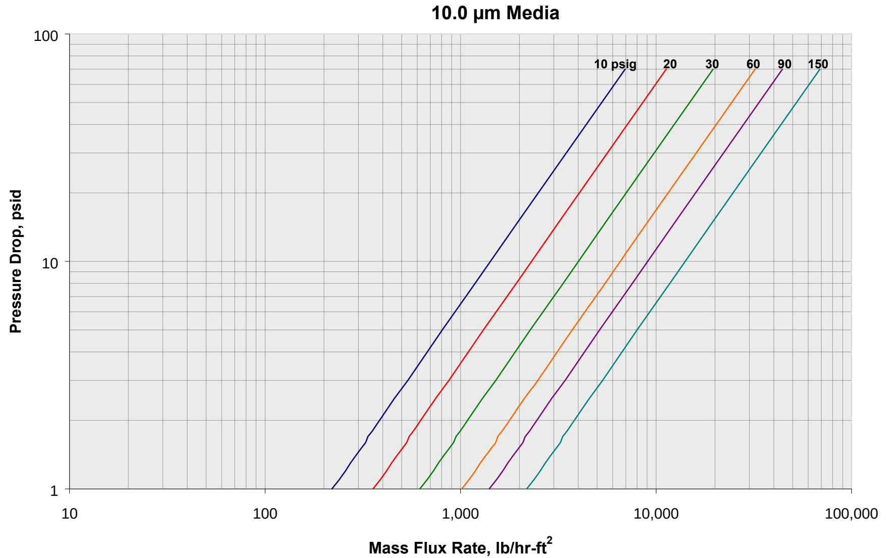
Figure 8: Media Pressure Drop by Steam Pressure
