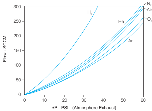
500 SCCM @ 30 psi N 2 Restrictor
